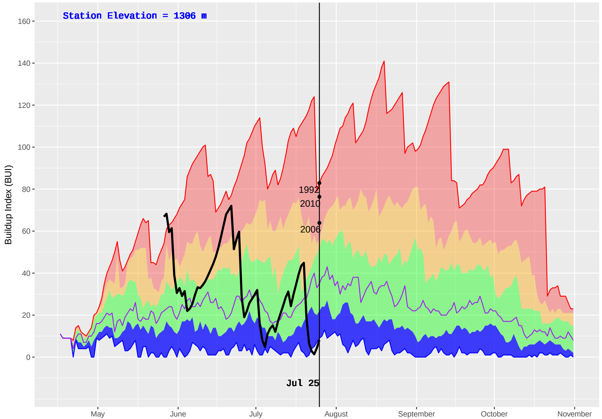
RED DEER (138) : Historical (1988–2016) and Current (2018) Noon Buildup Index (BUI)
