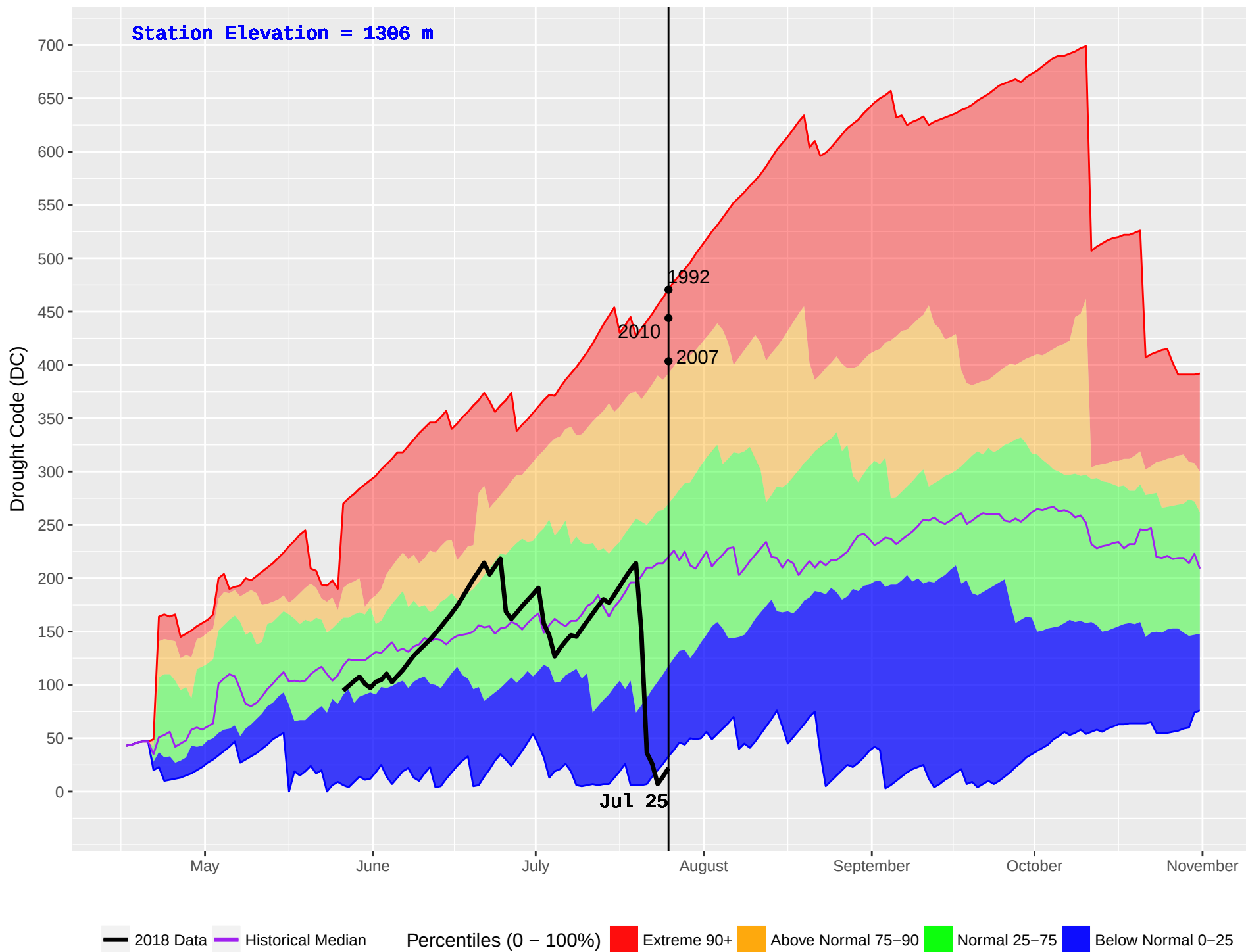
RED DEER (138) : Historical (1988–2016) and Current (2018) Noon Drought Code (DC)
